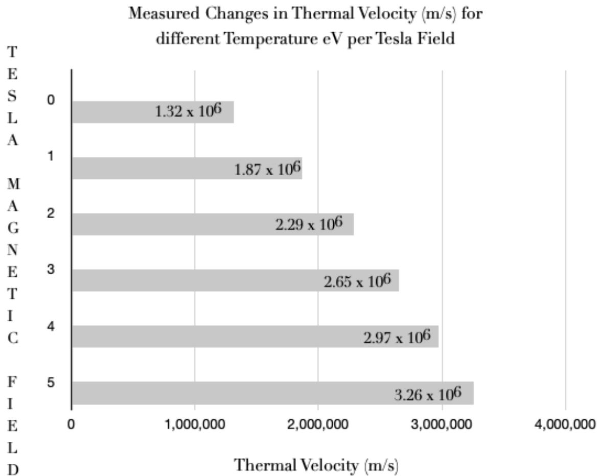
Graph 2. Changes in thermal particle velocity seen in associated increase in Tesla electromagnetic field strength.
