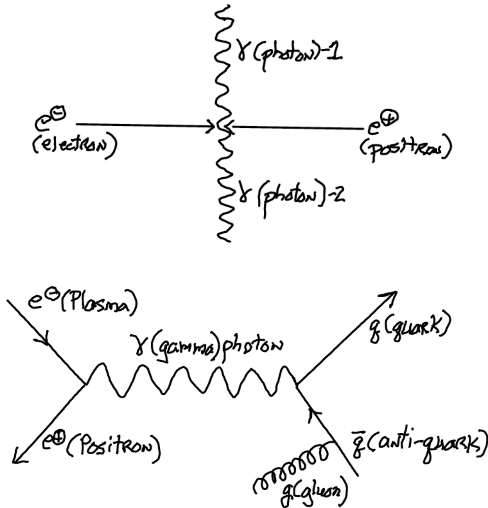
Figure 2: Theoretical models of positron-plasma interaction
